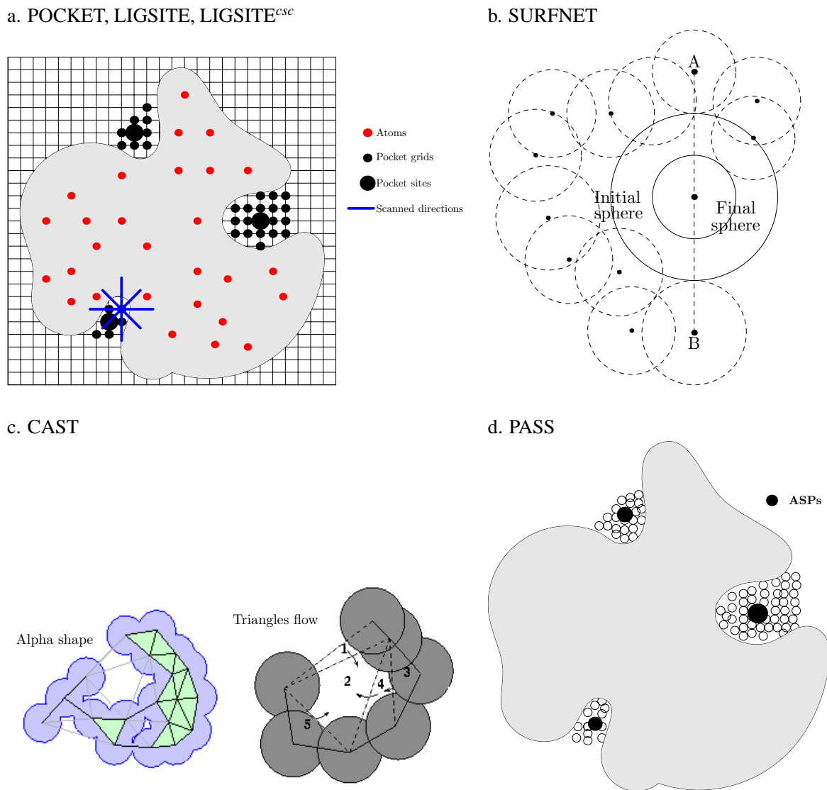
Figure 1 Pocket identification methods. a. POCKET, LIGSITE, and LIGSITE csc scan the grid for protein-solvent-protein and surface-solvent-surface events, respectively. POCKET uses 3, LIGSITE and LIGSITE csc 7 directions. POCKET and LIGSITE use atom coordinates while LIGSITE csc uses the Connolly surface. b. SURFNET places a sphere, which must not contain any atoms, between two atoms. The spheres with maximal volume define the largest pocket. c. CAST triangulates the surface atoms and clusters triangles by merging small triangles to neighbouring large triangles. d. PASS coats the protein with probe spheres, selects probes with many atom contacts, and then repeats coating until no new probes are kept. The pockets, or active site points, are the probes with large number of atom contacts.
